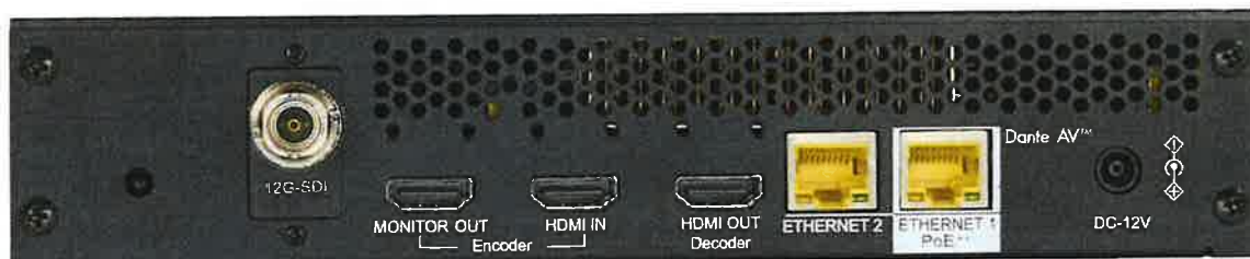
Back Panel (D20S)
