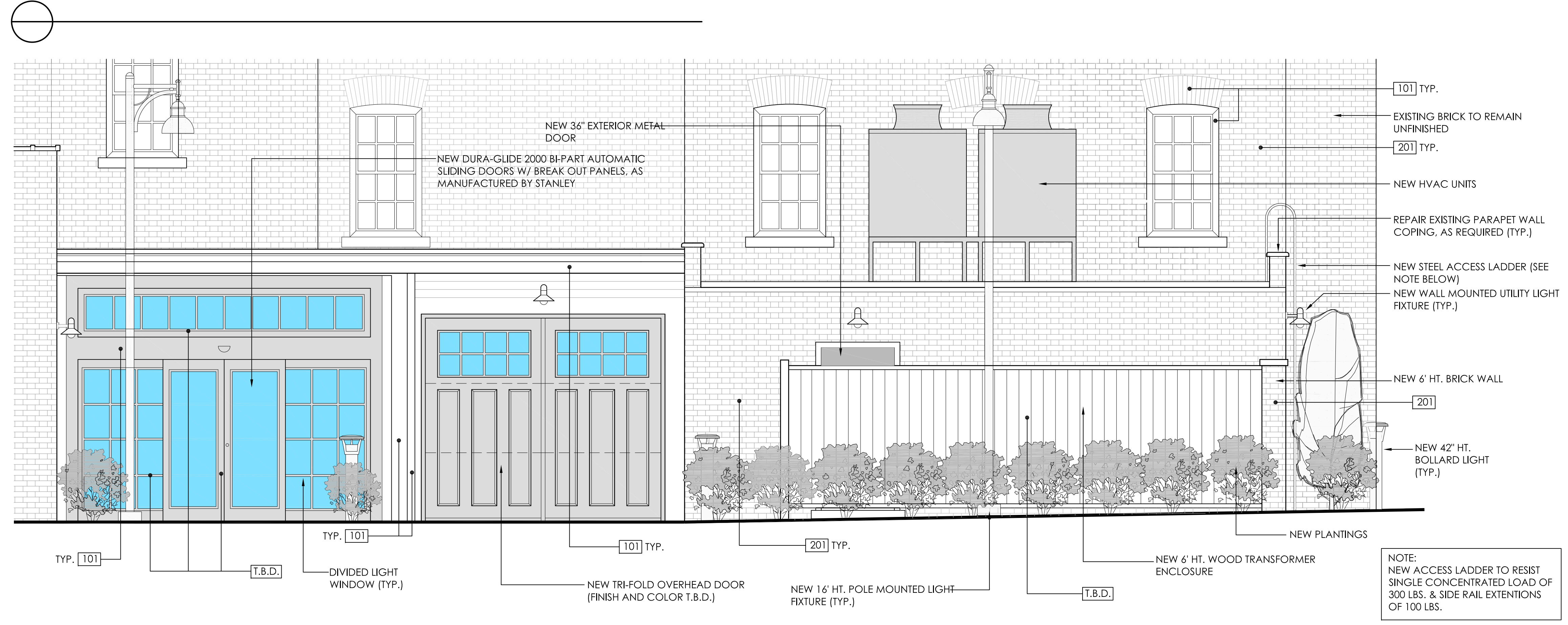
2 PROPOSED SIDE ELEVATION (SECONDARY LOBBY ENTRANCE) SCALE: 3/8"=1'-0"
