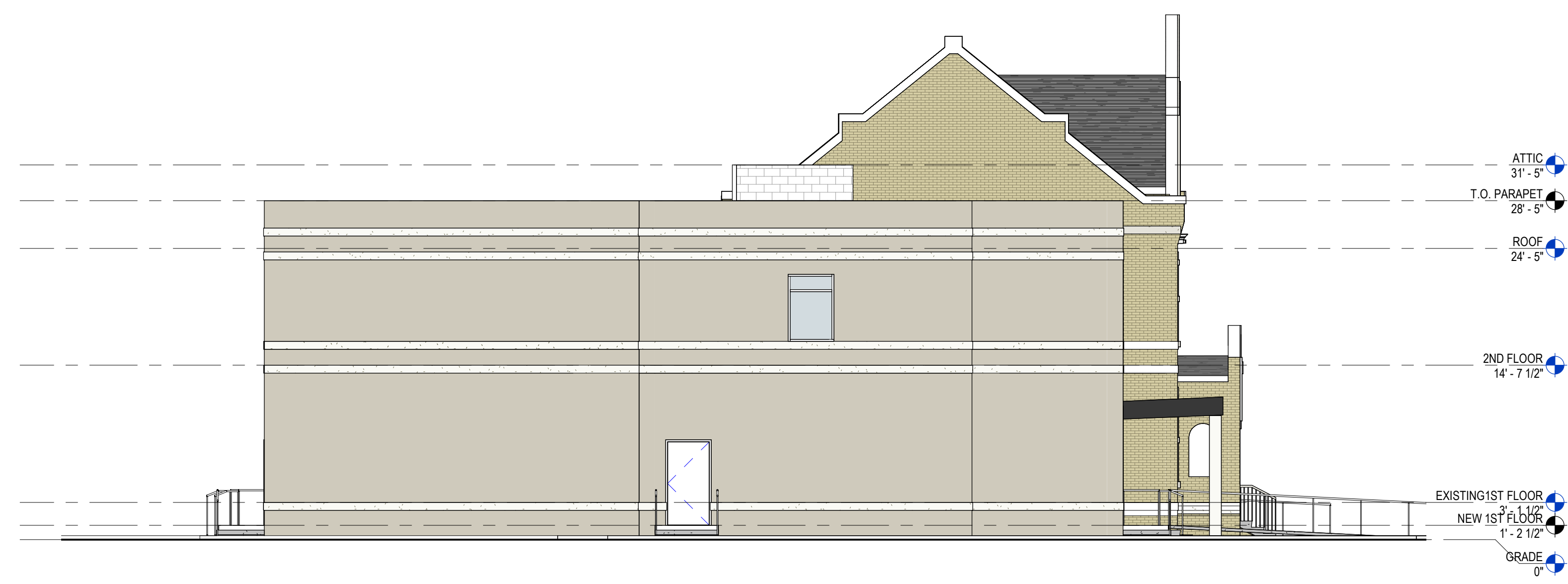
3 WEST ELEVATION 1/8" = 1'-0"
