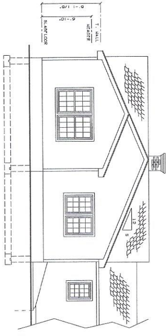
PARTIAL PROPOSED REAR ELEVATION SCALE: 1/4" = 1'-0"
