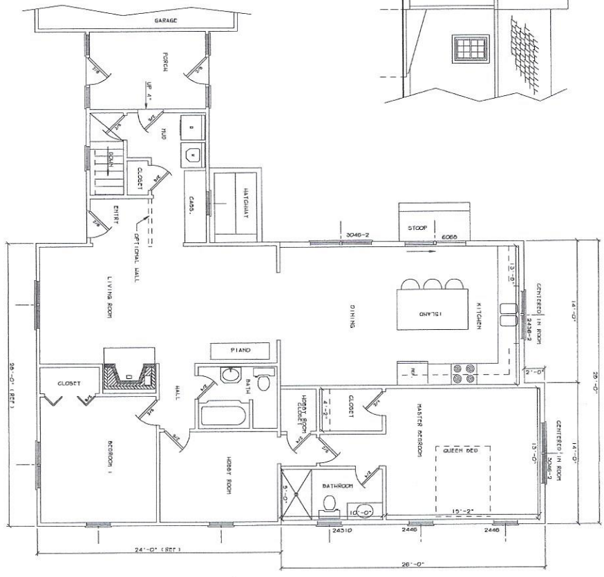
PROPOSED FLOOR PLAN SCALE: 1/4" = 1'-0"
