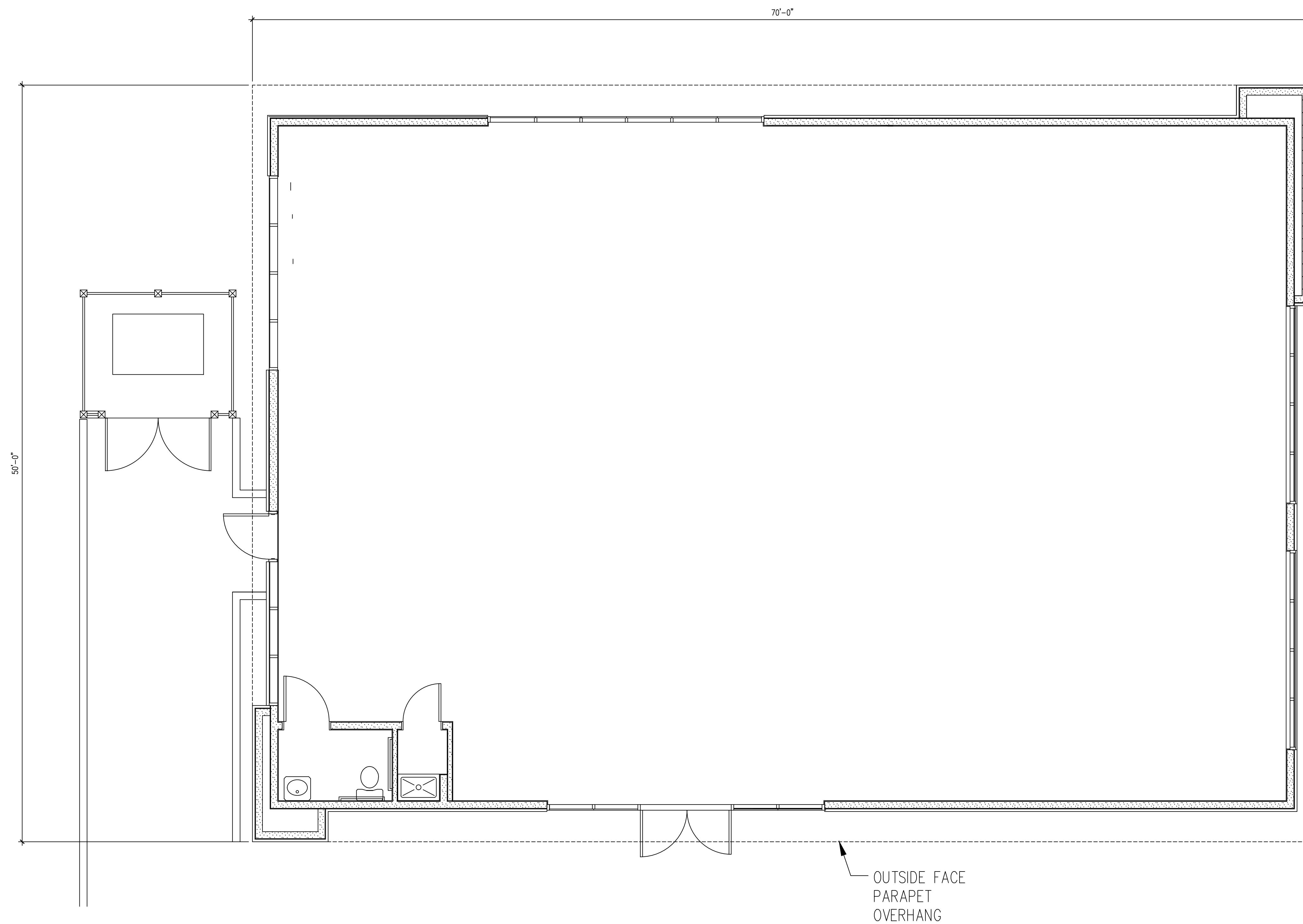
Floor Plan
